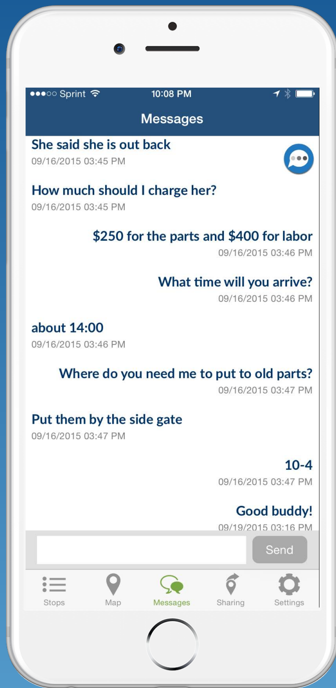
Dispatcher Messaging
